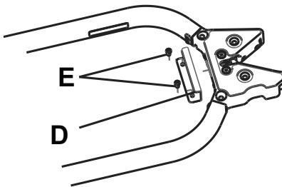
Figure 11 – Catch plate
